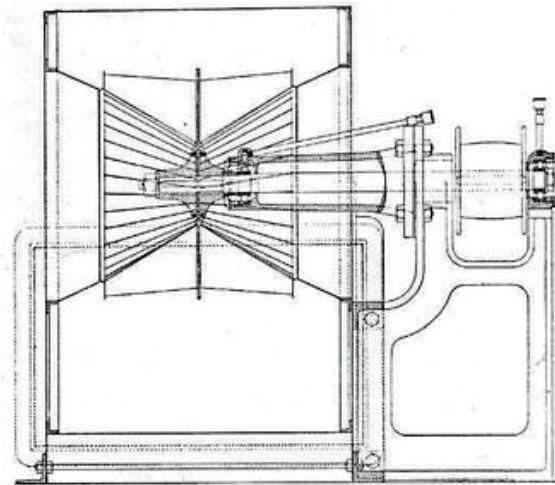
Fig. 10. Transverse Section through Fan Case. Longitudinal Section through Fan Wheel Blades. Double Air-Inlet Fan, Belt-driven.
