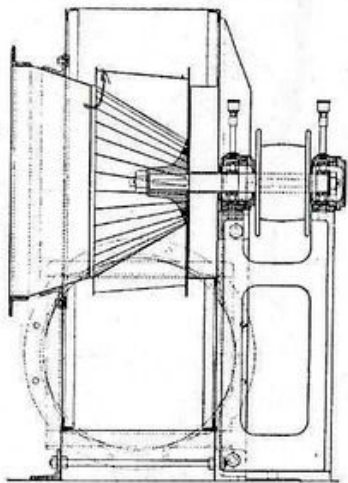
Fig. 8. Transverse Section through Fan Case. Longitudinal Section through Fan Wheel Blades. Single Air-Inlet Keith Fan, Belt-driven.
